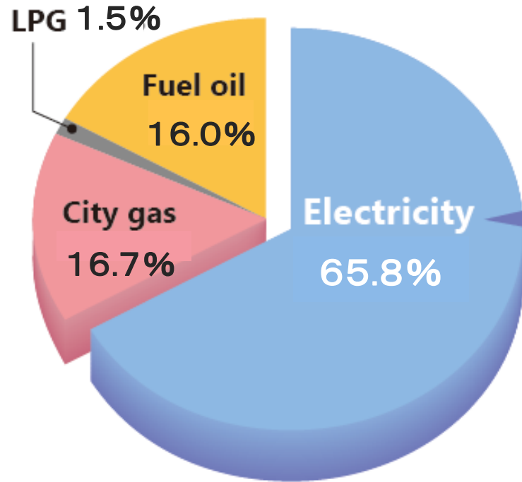
Breakdown of energy-related CO 2 emissions in Tokyo (preliminary results for FY 2020)
