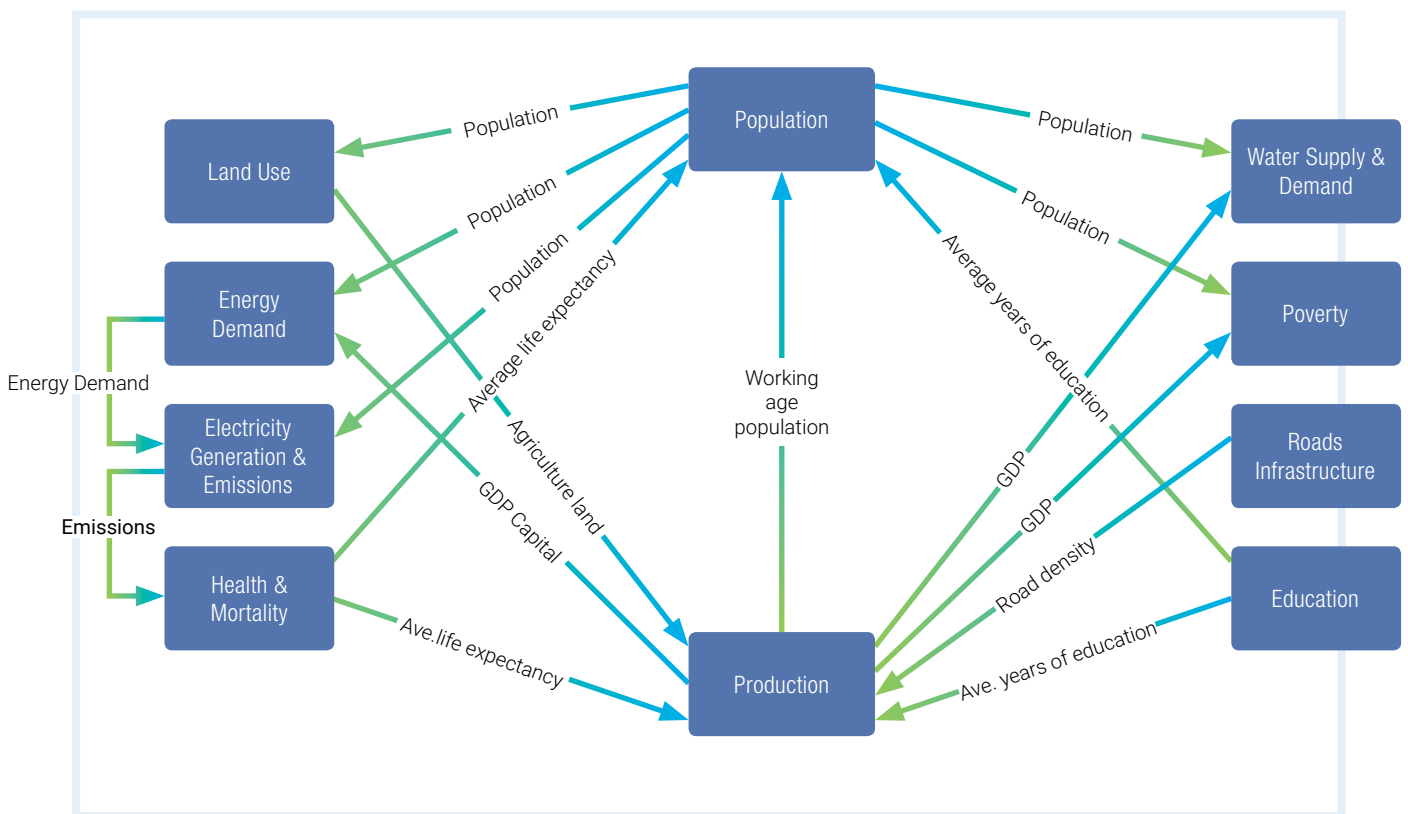
Figure 7: Macro structure of the core SD model
