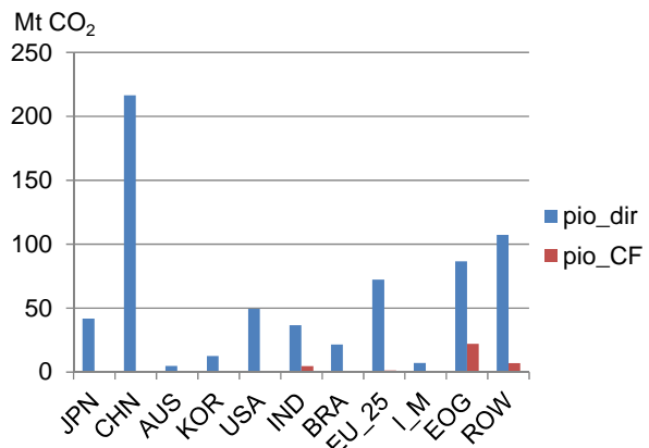
Figure A4 Direct emissions and CFs of pig iron sector
