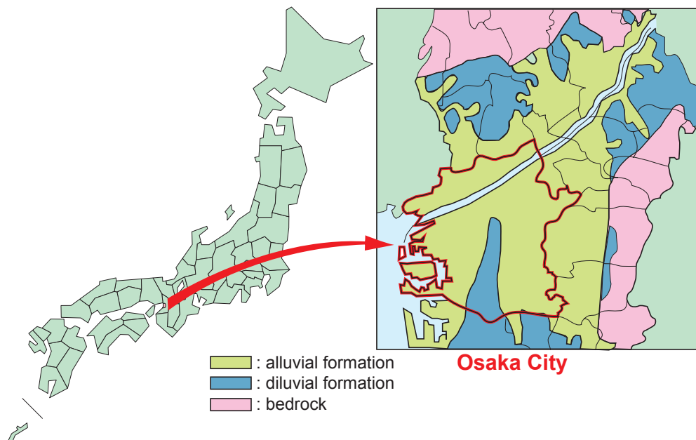
Figure 1. Location of Osaka and its Geological Characteristics
